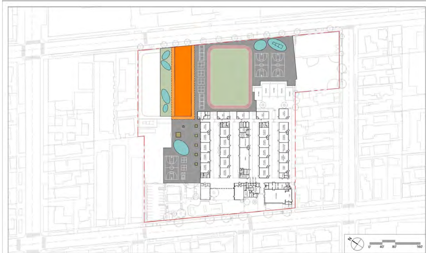
PHASE 1 - PROJECT 1 NEW 1-STORY CLASSROOM BLDG AND FIELD
