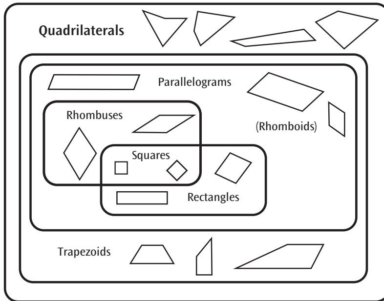
Figure 5-1. Classification of Quadrilaterals
